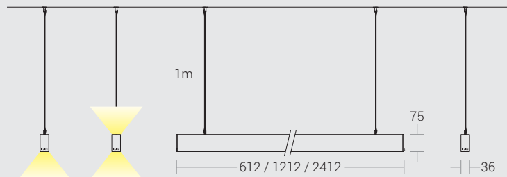
Dimension in mm
